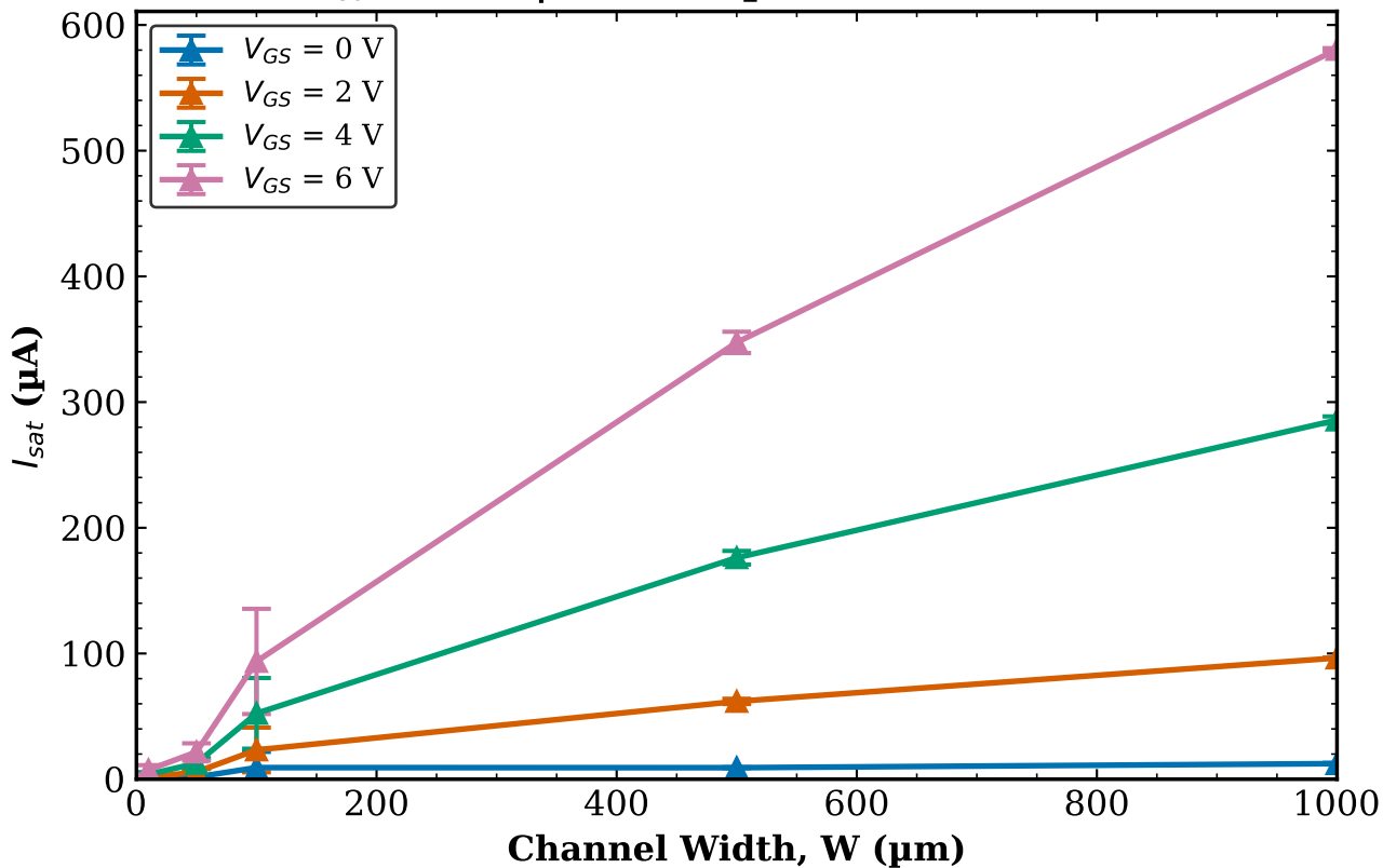
All Chips - Combined I_{sat} vs W | L = 10\text{ }\mu\text{m} (mean \pm std)
